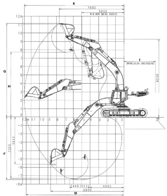
Level excavation with 10' 3" (3,13 m) arm
