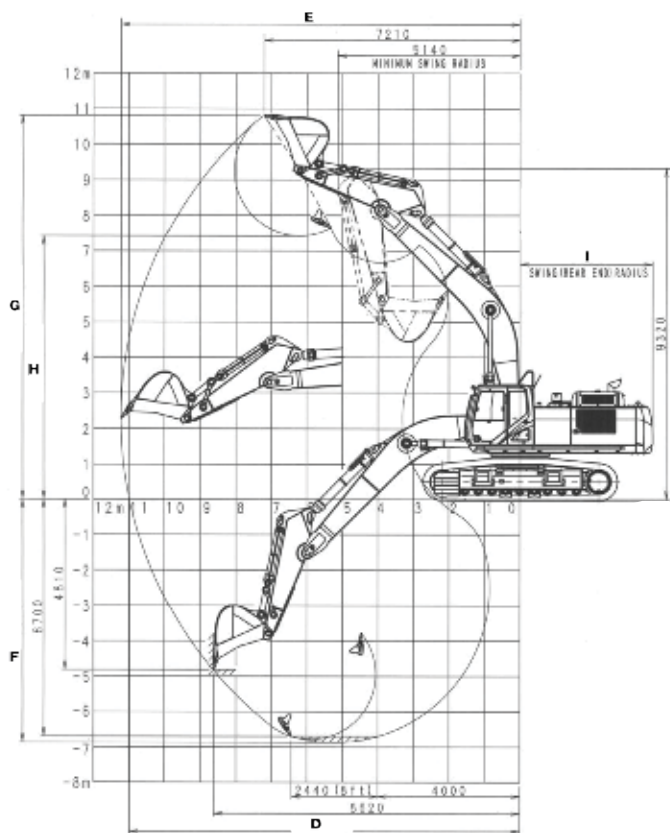
Level excavation with 8' 3" (2,53 m) arm
