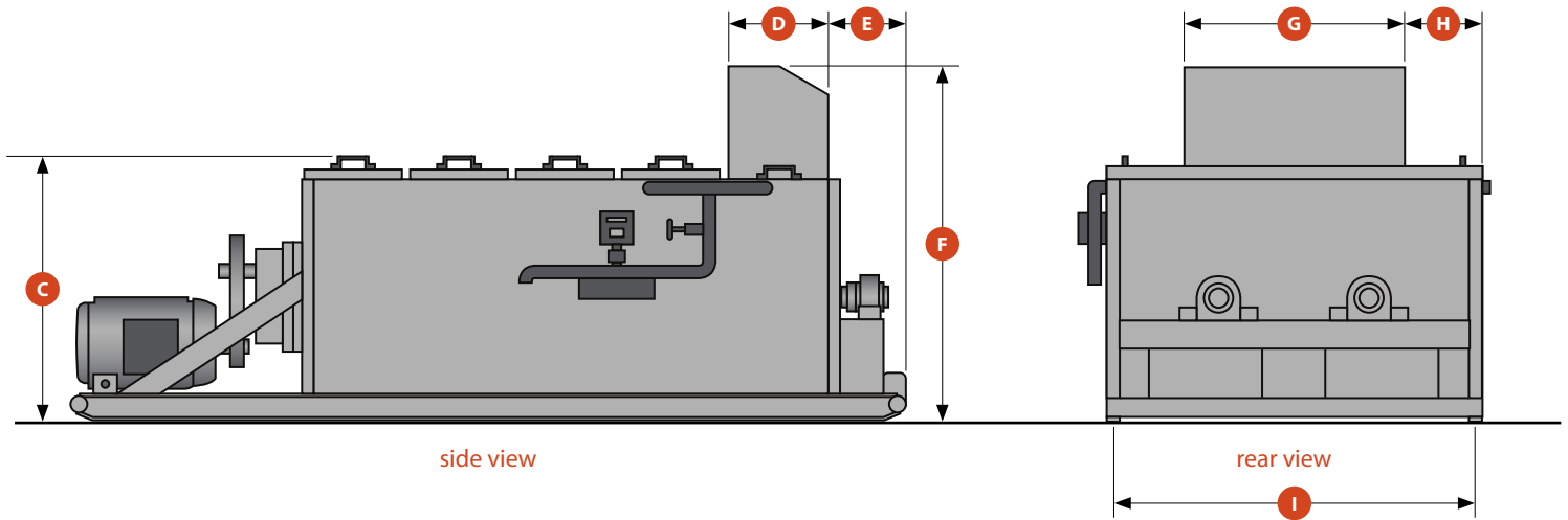
Pugmill Mixer Dimensions - Inches (mm)
